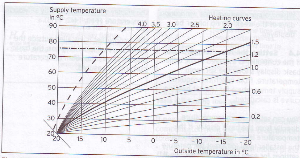
Fig. 4.1 Diagram Room Temperature Setting
